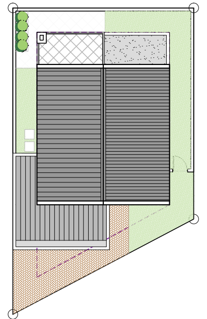
ROOF LAYOUT 1:200
